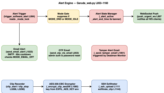
FIGURE 6. Alert engine dataflow. The mode gate short-circuits all downstream work during Do Not Disturb or Idle; the three asynchronous channels (WebSocket, SMTPS, AES-256-CBC encrypted clip upload) keep the slow paths off the inference thread, which is the precondition for the FPS-flatness result of Sec. VI-I.
