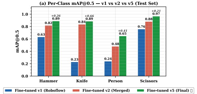
FIGURE 10. Per-class \text{mAP}@0.5 progression across v1, v2, and v5. Knife shows the largest single-class gain (+0.66); Scissors reaches the highest absolute score (0.967); Person remains the hardest class at 0.647. All four classes improve monotonically with dataset scale.
