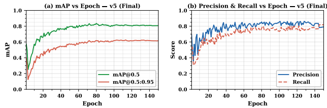
FIGURE 8. Validation metrics versus training epoch. The detector converges to a balanced precision-recall operating point with no sign of trade-off collapse.
