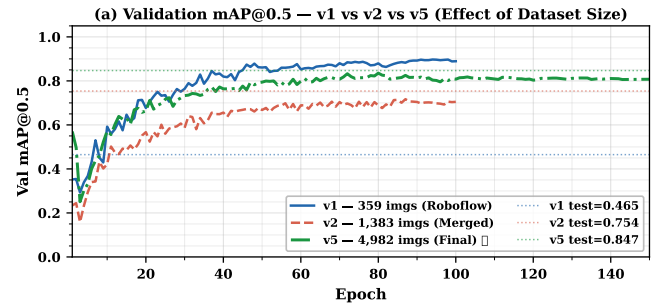
FIGURE 17. Validation mAP@0.5 progression against training-set size. v1 (359 images) converges to a deceptively high val mAP (~0.88) that does not transfer (test 0.465); v5 (4,982 images) converges to 0.817 val and 0.847 test. The trajectory is single-seed, single-split, and the v2→v5 additions are targeted at the weakest class (Section IV-A), so it is an empirical trajectory on one corpus rather than a randomised scaling law.
