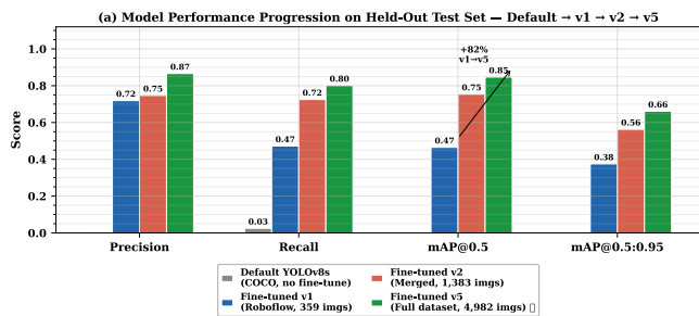
FIGURE 9. Four-model comparison on the held-out test set. COCO-pretrained YOLOv8s scores near zero on this four-class task; fine-tuning on 359 images (v1) recovers to 0.465 \text{mAP}@0.5 , the intermediate v2 (1,383 images) reaches 0.754, and v5 (4,982 images) reaches 0.847 — an 82% gain over v1 driven entirely by dataset growth.
